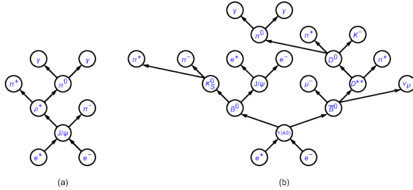
Figure 3.4: Topology diagrams of (a) e^+e^- \rightarrow J/\psi and (b) e^+e^- \rightarrow \Upsilon(4S) \rightarrow B^0 \bar{B}^0 , two typical processes at e^+e^- colliders, such as Belle II and BESIII
